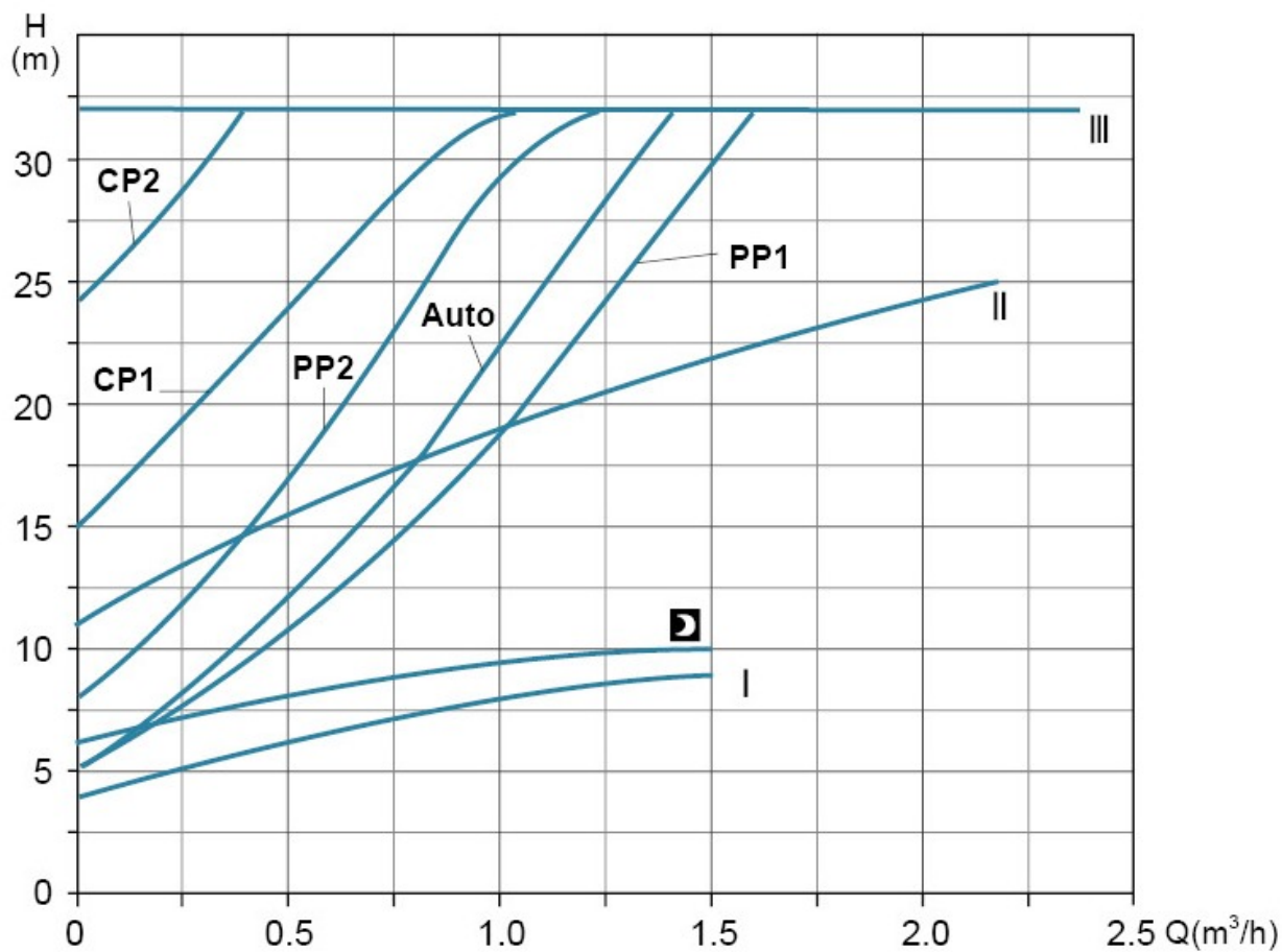
ARPXX-50 Q-H
