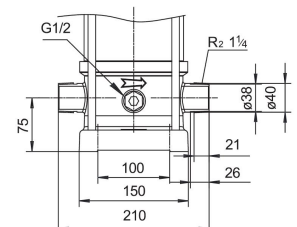
Threaded connection (/G)
